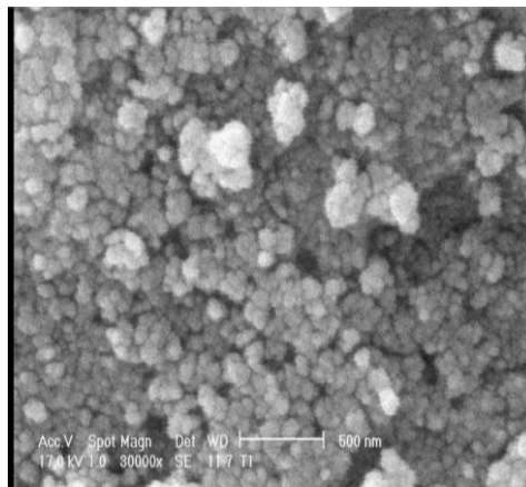
Fig.2. SEM photograph of the as-burnt ZnFe 2 O 4 powder.
