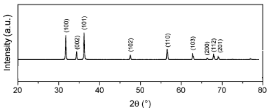
Fig.4. XRD patterns of \text{Zn}_{0.97}\text{Co}_{0.03}\text{O} photocatalysts
