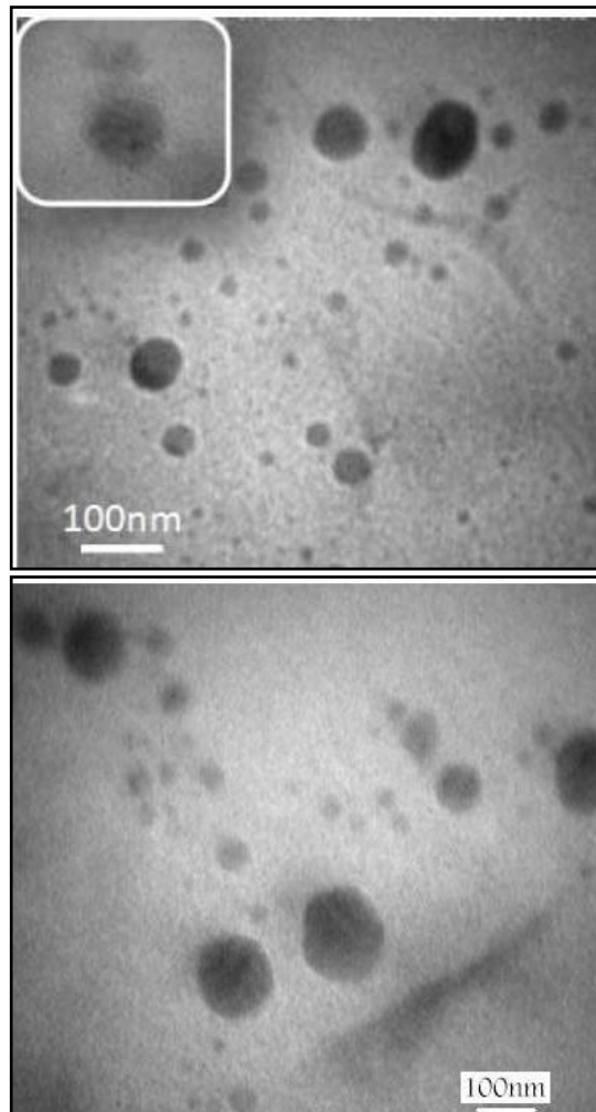
Fig. 5. TEM images of silver/copper alloy nanoparticles showing that the grains were formed by this method. The darker color of some parts of the grains shows that the grains contain more than one material, and thus the silver/copper alloy nanoparticles were formed.
