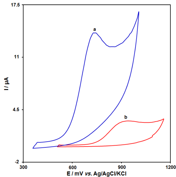
Fig. 2: Cyclic voltammograms of (a) CuO/SPE and (b) bare SPE in 0.1 M PBS (pH 7.0) in the presence of 40.0 \mu\text{M} amitriptyline at the scan rate 50 mVs -1 .
